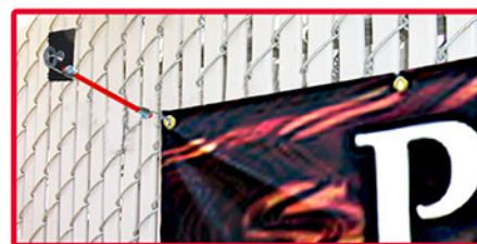
Mount Banners using Eye Bolts to Chain Link Fence by using SLK3000 LinkKlip and SLKLAMP LinkLamp with Eye Bolt to Clamp to fence
